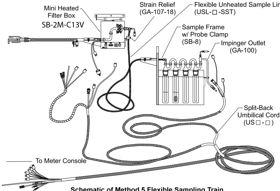
Schematic of Method 5 Flexible Sampling Train
